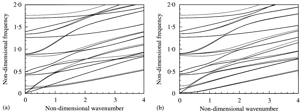
Figure 6. Dispersion curves for waves propagating in a (C0/G \pm 45)_s cylinder. (a) \beta = 0 ; (b) \beta = 30^\circ . —, wet cylinder; ---, dry cylinder.
